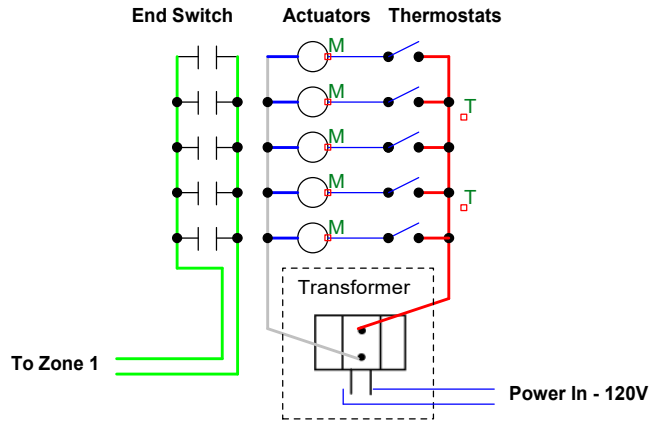
Schematic Diagram - 5 Thermostats, 5 Zone Valves
